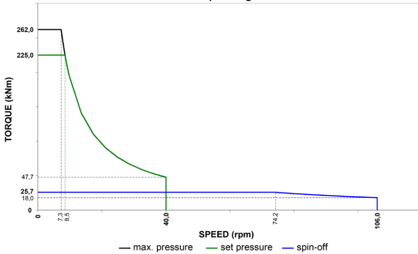
Torque Diagram
